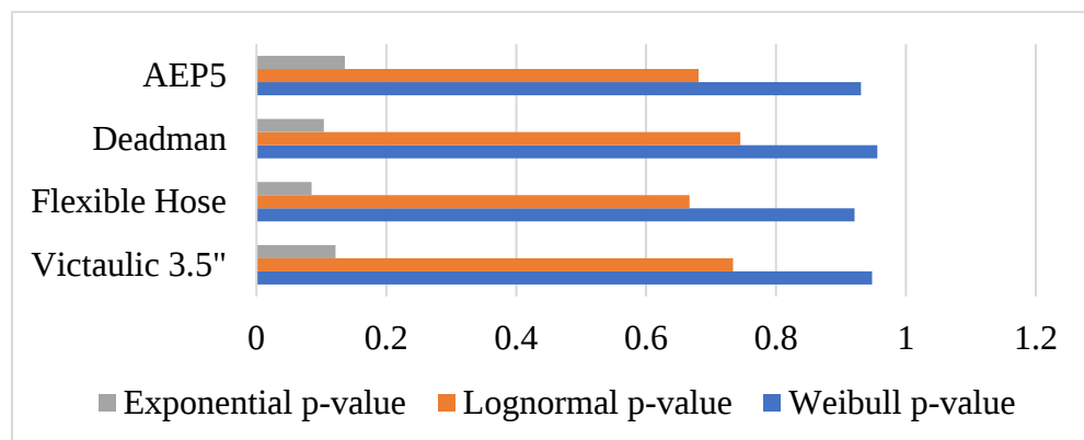
Figure 4. P-Value Kolmogorov-Smirnov Compare
